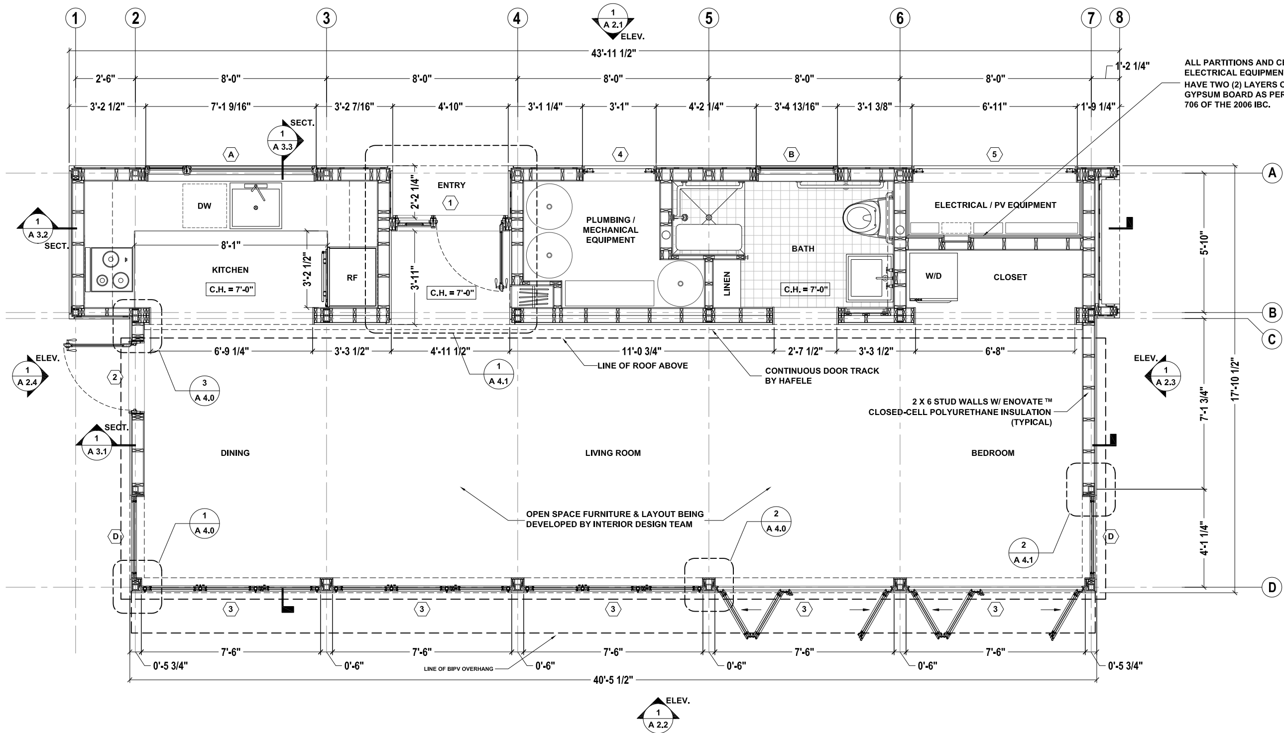
ARCHITECTURAL FLOOR PLAN SCALE 1/4" = 1'-0" 0 2' 4' 8'
